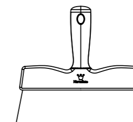
50RAS06 Total size: 180x200 mm Handle: h 130x189,7 mm Lama - Blade 200 x h 50 mm
